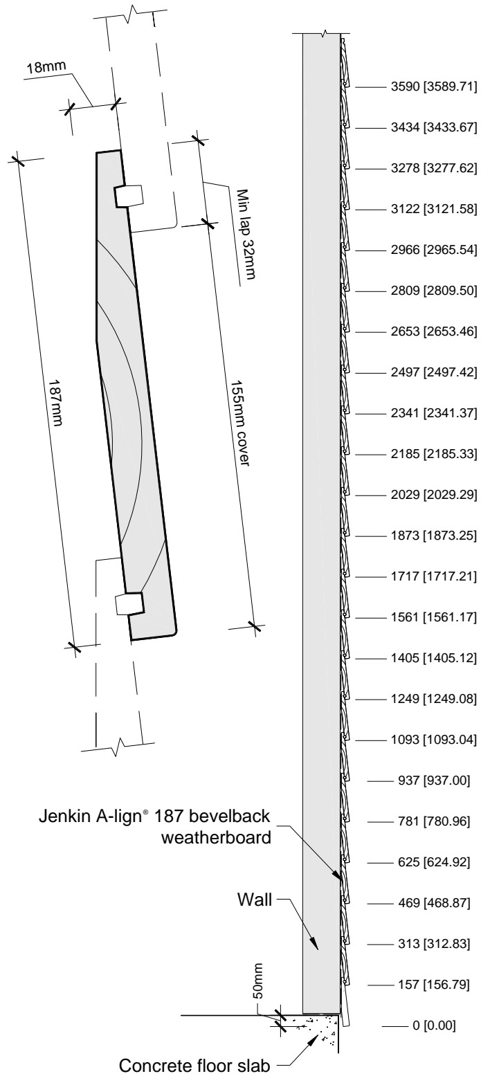
Jenkin A-lign® 187 bevelback weatherboard
