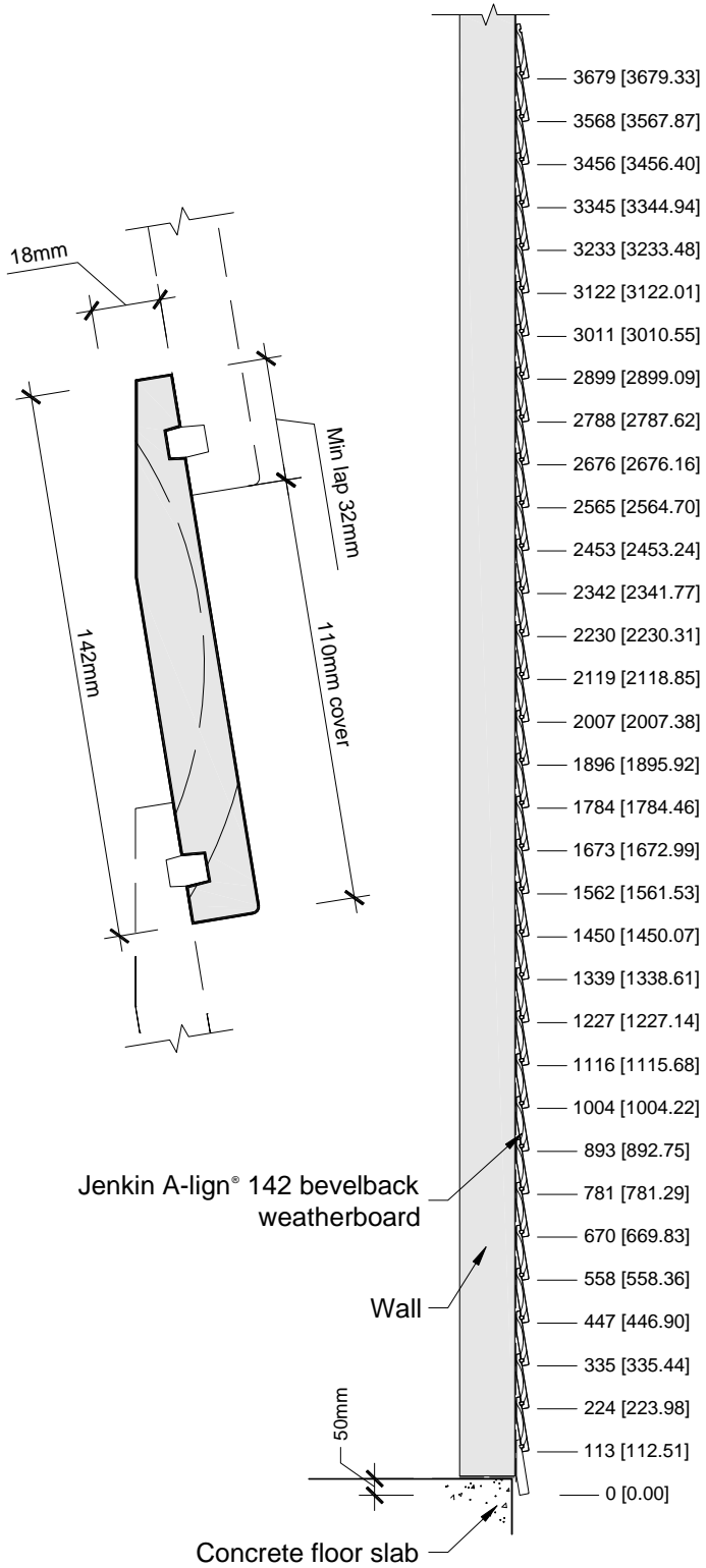
Jenkin A-lign® 142 bevelback weatherboard
